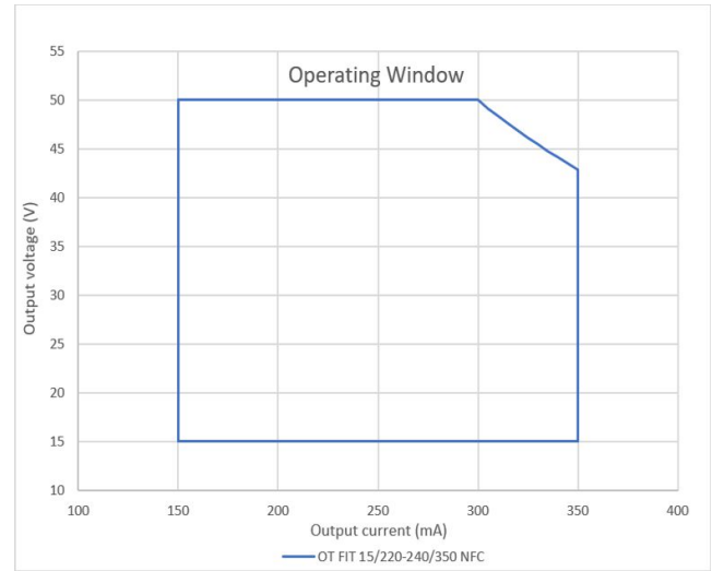
OT FIT 15 NFC G2 Operating window
